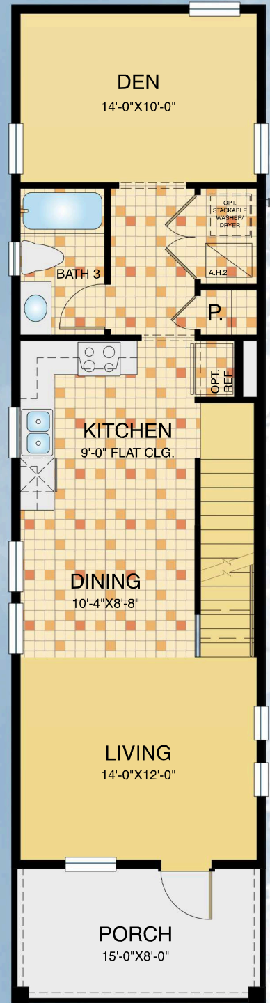
2ND FLOOR PLAN
